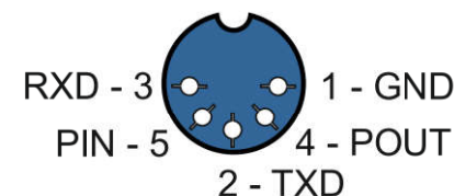
Serial view on female socket
